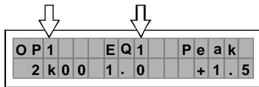
Example: Output 1-Filter 1
