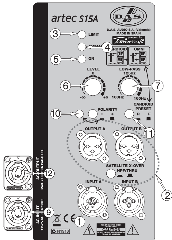
Amplifier of artecS15A
